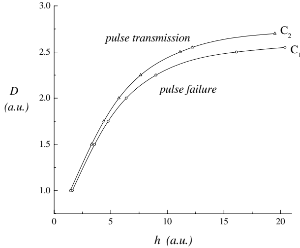
Fig. 8. Diagram of pulse driving by single-pin contact in (D, h) parameter plane. The pulse fails to propagate for values chosen below the curve C_1 . Above the curve C_2 the pulse successfully overcomes the contact. Units are arbitrary (a.u.).
