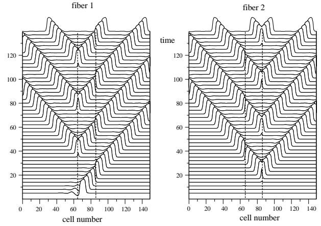
Fig. 9. A generator of synchronized pulses when the parallel excitable fibers have two-pin contacts. Parameter values: \alpha = 4.5 , D = 2 , h_{65} = h_{85} = 5 . Vertical axes account for time in arbitrary units (a.u.).
