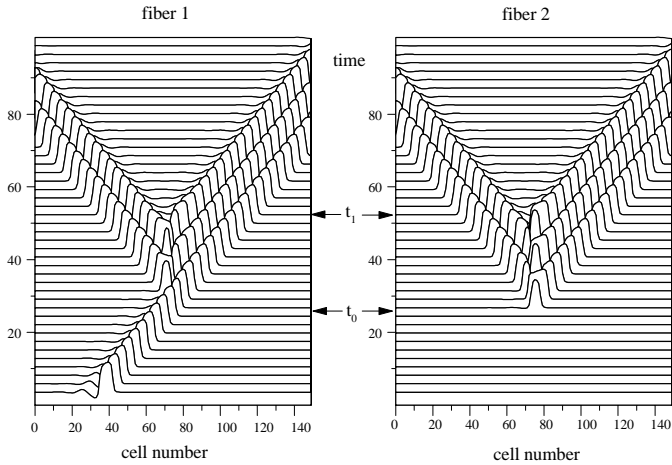
Fig. 5. Long lasting pulse source generating trains of pulses. Parameter values: \alpha = 4.5 , D = 2 , h = 1.05 , t_0 = 25, t_1 \approx 52 . Vertical axes account for time in arbitrary units (a.u.).
