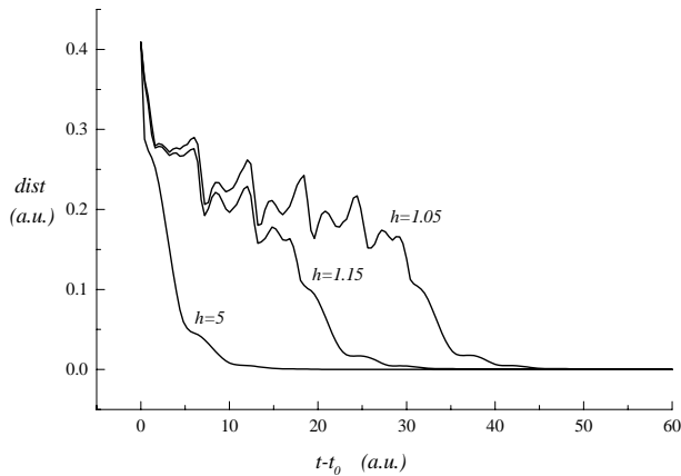
Fig. 6. Controlled distance, dist , as a function of time for three different values of the inter-fiber interaction. The curves illustrate that synchronization is indeed achieved. Units are arbitrary (a.u.).
