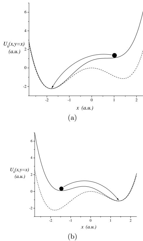
Fig. 3. Effective potential functions, U_h , for the coupled fibers describing (a) front acceleration and (b) front reversal propagation. Units are arbitrary (a.u.).
