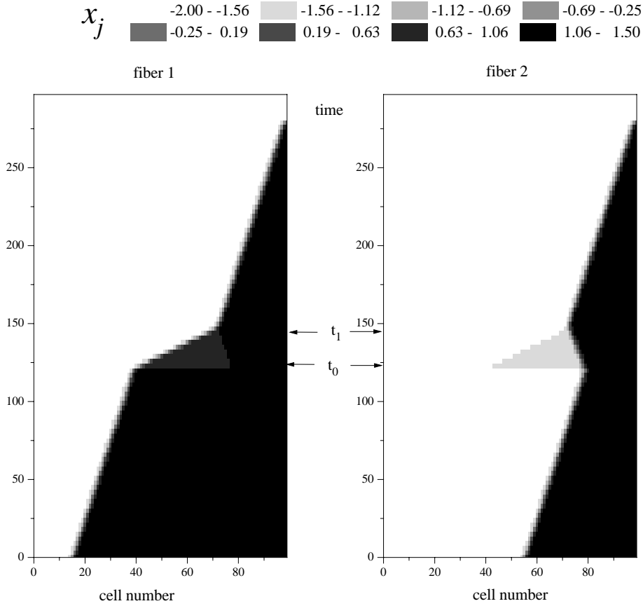
Fig. 2. Wave fronts in two identical bistable fibers with D = 2 . (a) Synchronization of two wave fronts traveling with finite time delay. For t < t_0 = 120 the chains are independent, h = 0 . At t = t_0 , the interaction is switched-on, t > t_0 , h = 0.5 . The time interval t_0 < t < t_1 \approx 140 corresponds to a transient process. Vertical axes account for time in arbitrary units (a.u.).
