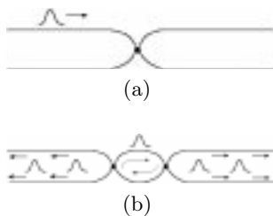
Fig. 7. Schematic diagram of two parallel fibers coupled by (a) a single-pin contact and (b) a double-pin contact.
