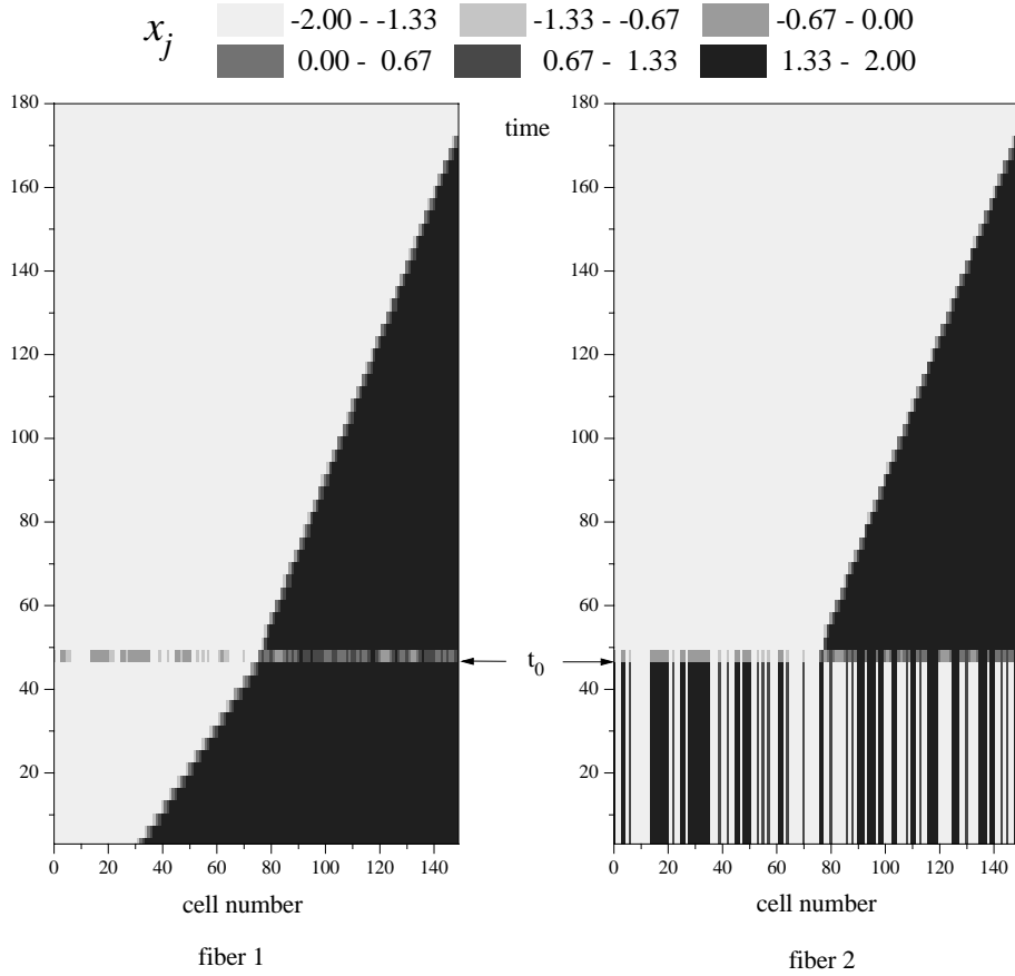
Fig. 4. Propagation failure overcome in coupled bistable fibers. Diffusion coefficients: D_1 = 3 , D_2 = 0.2 . At t_0 = 48 the inter-fiber interaction is switched-on, h = 10 . Vertical axes account for time in arbitrary units (a.u.).
